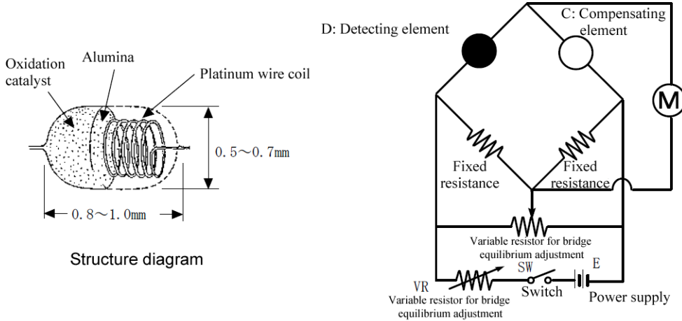
Basic circuit
